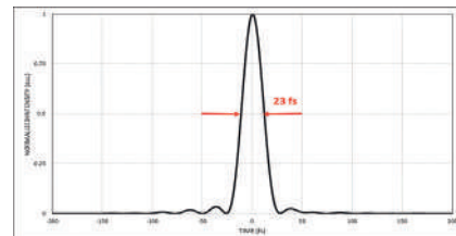
Pulsar 250 typical Wizzler pulse width measurement
